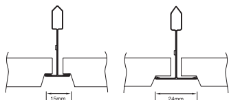
Angled Tegular with Supratine Grid
