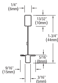
INTERLUDE Main Beam
